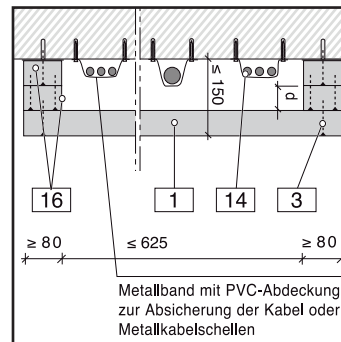
[6] Wand-/deckennahe Montage h ≤ 150
