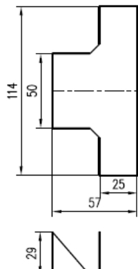
CROSS CONNECTOR TYPE B
