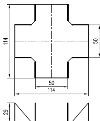
CROSS CONNECTOR TYPE A
